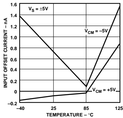
Figure 41. Input Offset Current vs. Temperature, V_S = \pm 5\text{ V}
