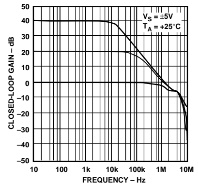
Figure 46. Closed-Loop Gain vs. Frequency, V_S = \pm 5\text{ V}
