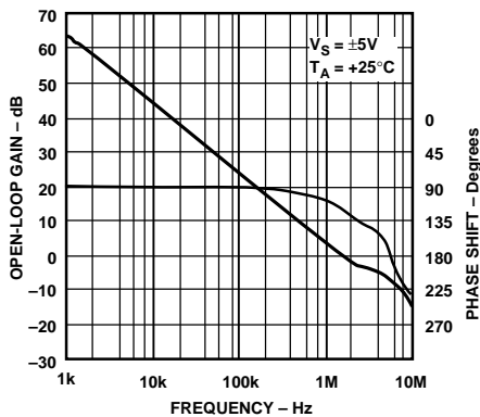
Figure 44. Open-Loop Gain & Phase vs. Frequency, V_S = \pm 5\text{ V}
