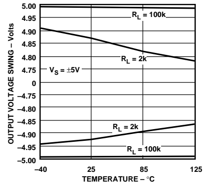
Figure 43. Output Voltage Swing vs. Temperature, V_S = \pm 5\text{ V}
