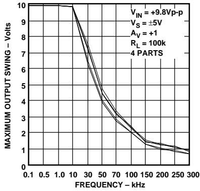
Figure 38. Maximum Output Swing vs. Frequency, V_S = \pm 5\text{ V}
