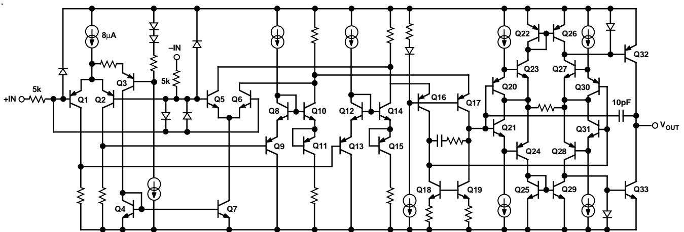
Figure 55. Simplified Schematic
