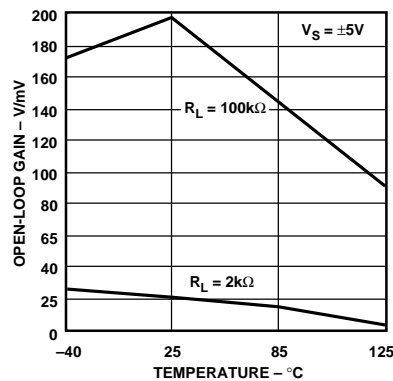
Figure 45. Open-Loop Gain vs. Temperature, V_S = \pm 5\text{ V}
