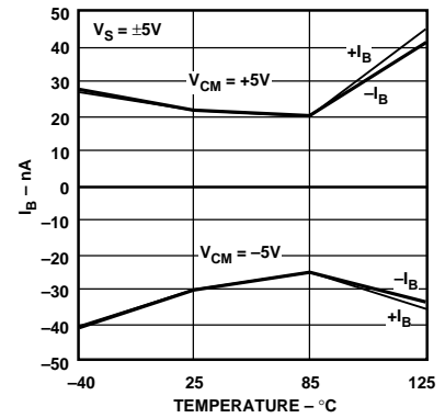
Figure 40. Input Bias Current vs. Temperature, V_S = \pm 5\text{ V}
